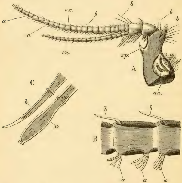
FIG. 26.— Astacus fluviatilis .—A, the right antennule seen from the inner side ( \times 5 ) ; B, a portion of the exopodite enlarged ; C, olfactory appendage of the exopodite ; a , front view ; b , side view ( \times 300 ) ; a , olfactory appendages ; au , auditory sac, supposed to be seen through the wall of the basal joint of the antennule ; b , setae ; en , endopodite ; ex , exopodite ; sp . spine of the basal joint.
